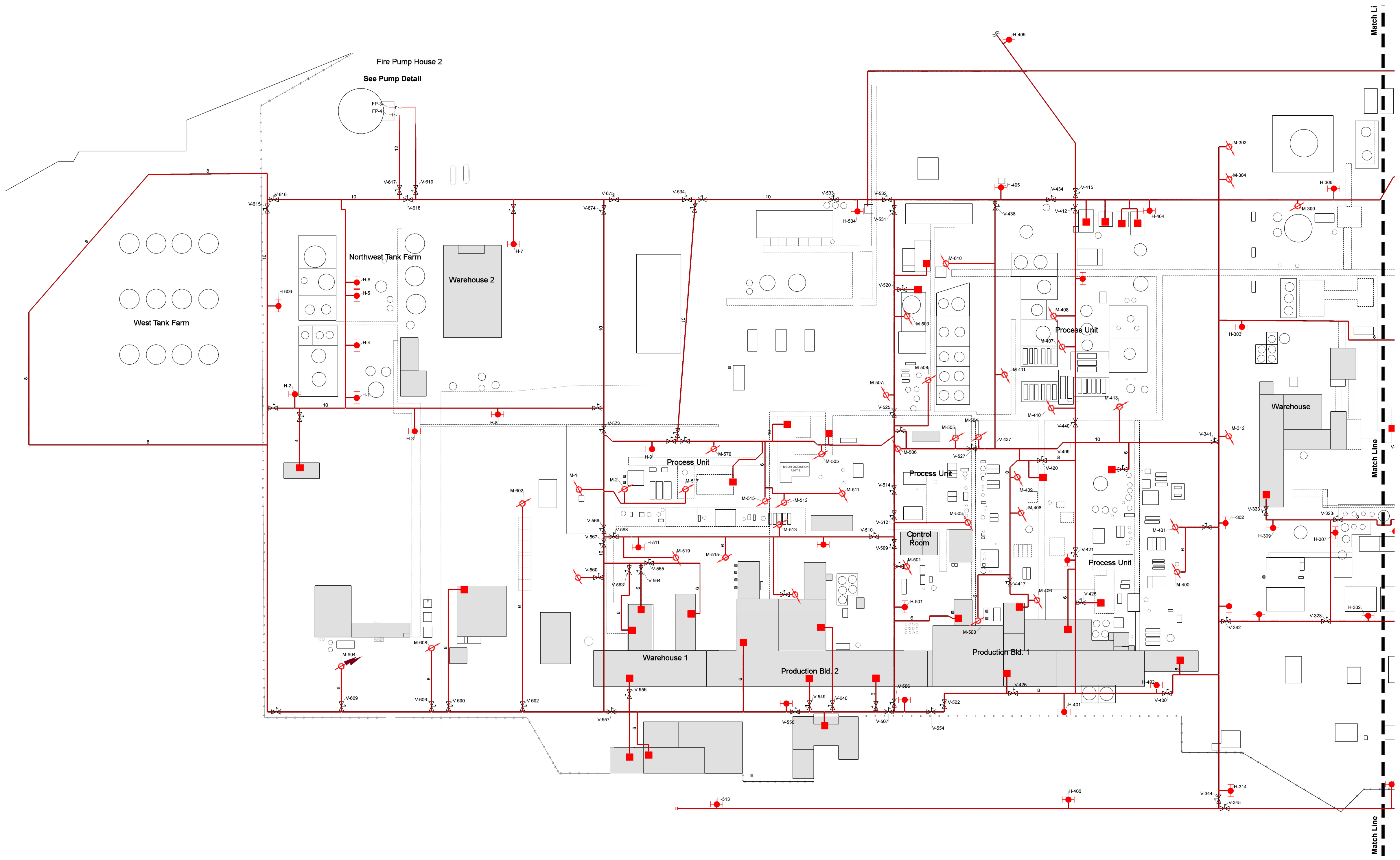
FIRE WATER PLOT PLAN
